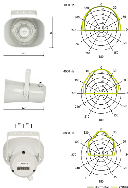
FREQUENCY RESPONSE
