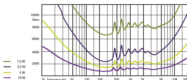
IMPEDANCE
